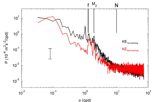
Fig. 9. Spectra of kinetic energy based on the ADCP data of the first (black line) and second (red line) mooring deployments. f indicates the local inertial period ( \sim 18.8 \text{ h} ), M_2 the semidiurnal tide ( \sim 12.4 \text{ h} ) and N indicates the buoyancy frequency computed from the CTD-data. (For interpretation of the references to color in this figure legend, the reader is referred to the web version of this article.)
