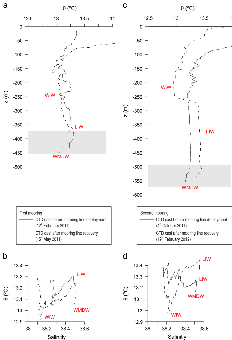
Fig. 2. Potential temperature profiles and T–S diagrams from CTD-data before the mooring deployment (solid line) and after the mooring recovery (dashed line), near the first (a and b) and the second (c and d) mooring locations. LIW: Levantine Intermediate Water; WIW: Western Mediterranean Intermediate Water; WMDW: Western Mediterranean Deep Waters.
