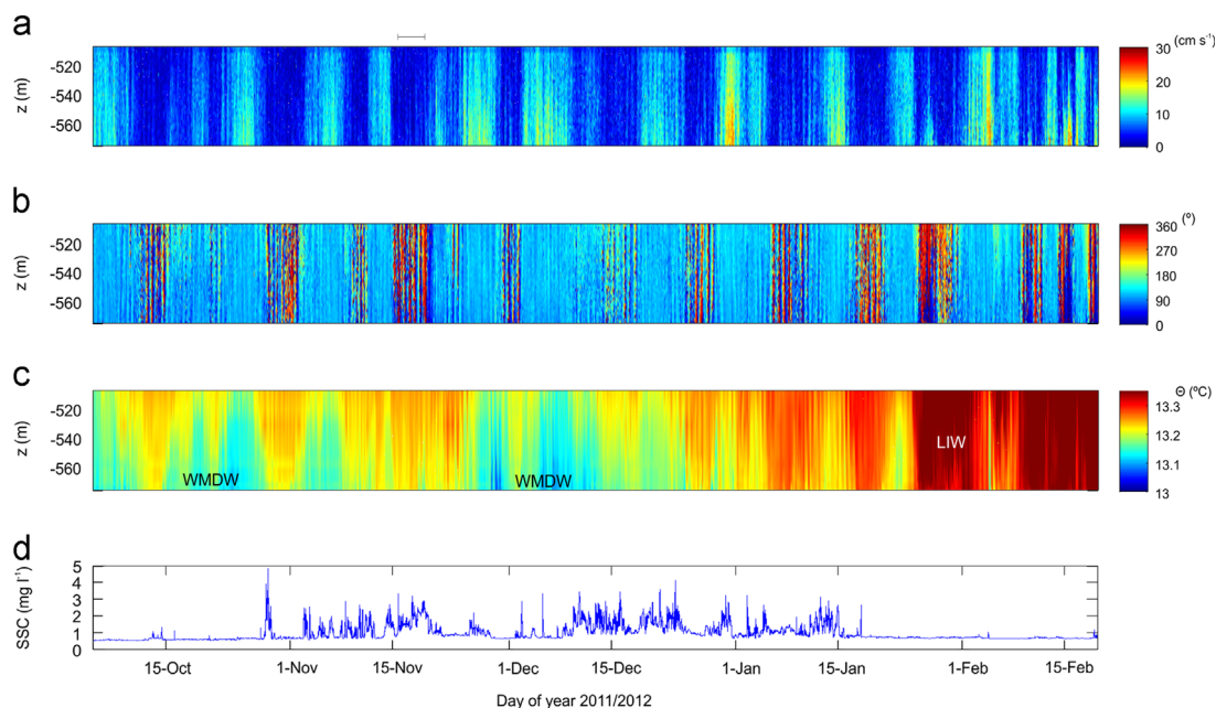
Fig. 4. As Fig. 3, but for the second mooring.
