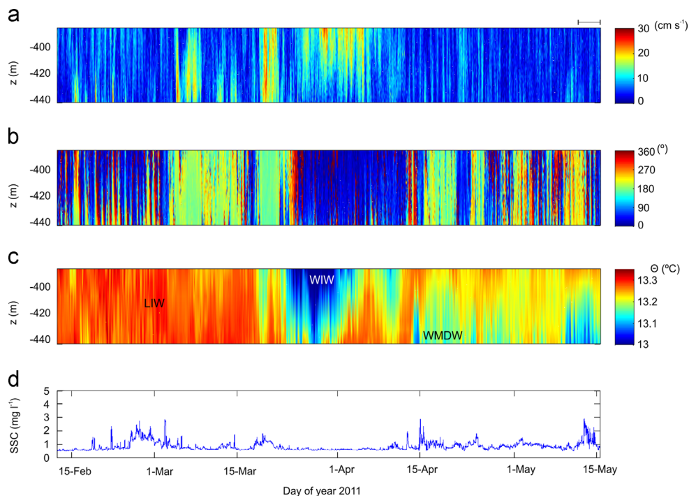
Fig. 3. (a) Current magnitude ( cm s^{-1} ), (b) current direction ( ^\circ ) from ADCP, and (c) potential temperature and (d) near-bottom turbidity records from the OBS, from the first mooring. LIW: Levantine Intermediate Water; WIW: Western Mediterranean Intermediate Water; WMDW: Western Mediterranean Deep Waters.
