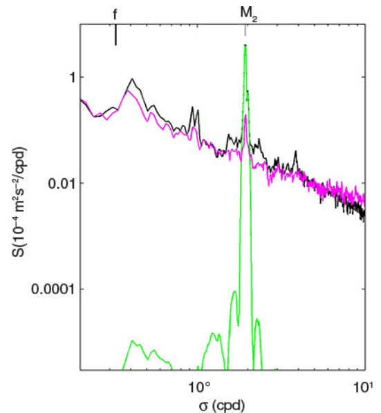
Fig. 3. Example of kinetic energy spectrum from a 1-yr current meter record at 105 mab in KG, including semidiurnal band-pass filter (green) and vertical difference spectrum from 5 to 210 mab (purple).
