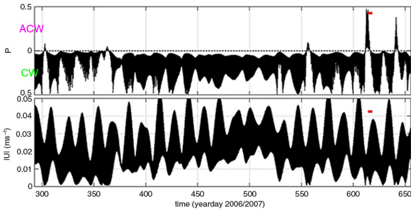
Fig. 4. One year time series of typical deep CB semidiurnal polarisation direction, observed at 28.8^\circ\text{N} , 500 mab. The polarisation sign is anticlockwise when positive and clockwise when negative [arbitrary values between (-0.5, 0.5) ]. The red bar indicates a 4-d period of which hodographs are given in Fig. 5a. (b) Current amplitude.
