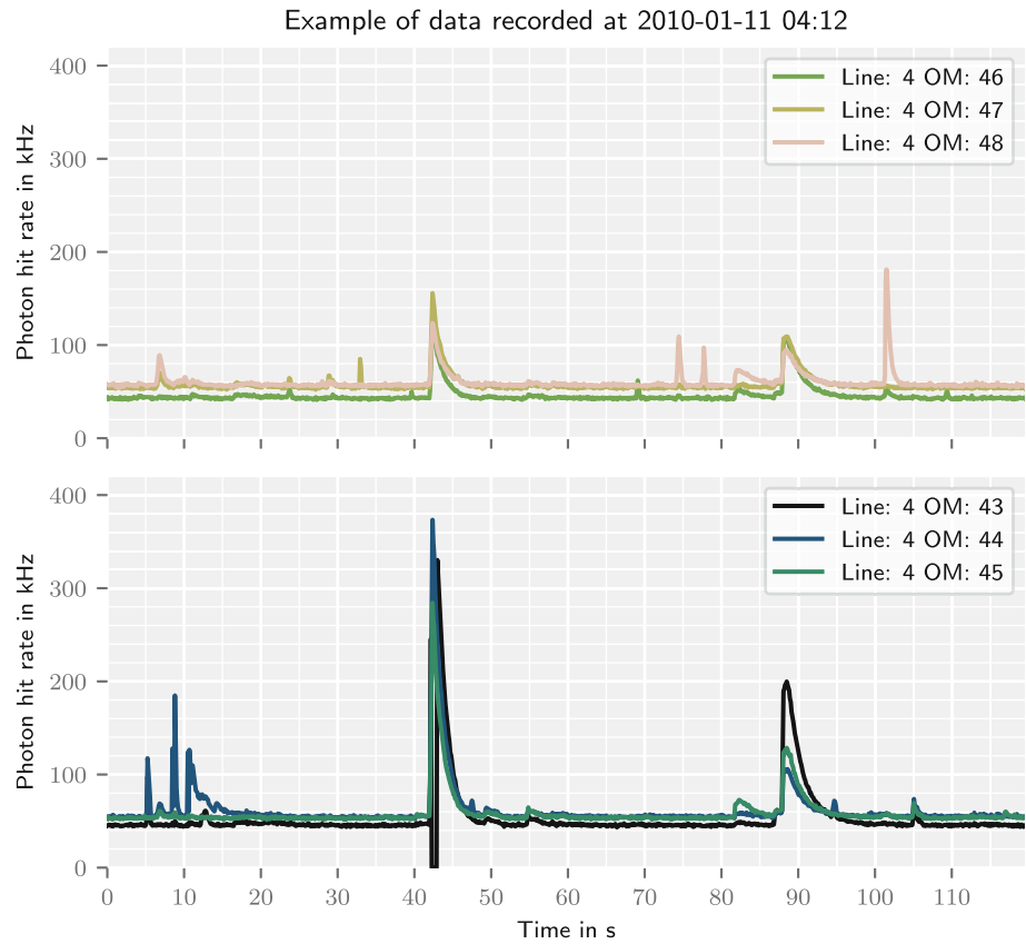
Fig. 2. Recorded photon hits of six OMs. The upper plot shows the photon hits of the optical modules in one storey. The lower plot shows the photon hits of the optical modules in the storey below.
