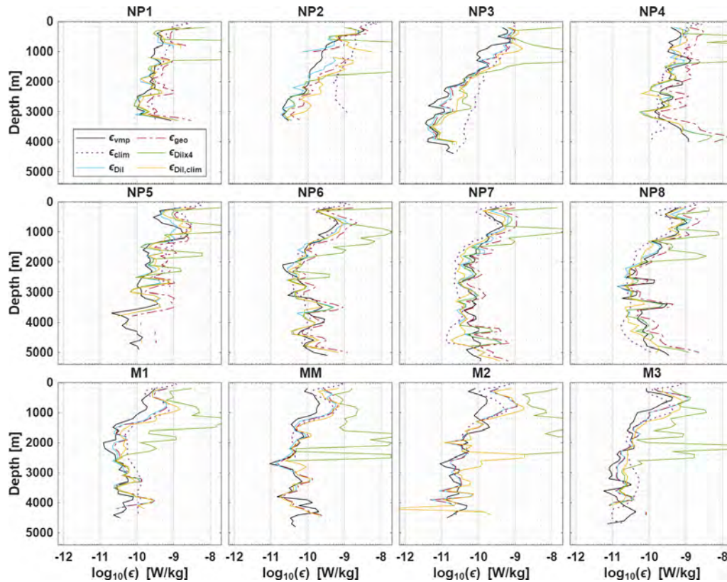
Figure 6. Dissipation estimates \epsilon_{TP} for all different methods ( \epsilon_{geo} : Method 1, \epsilon_{Dil} : Method 2, \epsilon_{Dilx4} : Method 3 and \epsilon_{Dil,clim} : Method 4, as defined in Sect. 5.4) are compared to \epsilon_{vmp} and the used climatological estimates \epsilon_{clim} . For plotting purposes all data is averaged over the same half overlapping 200 m bins.
