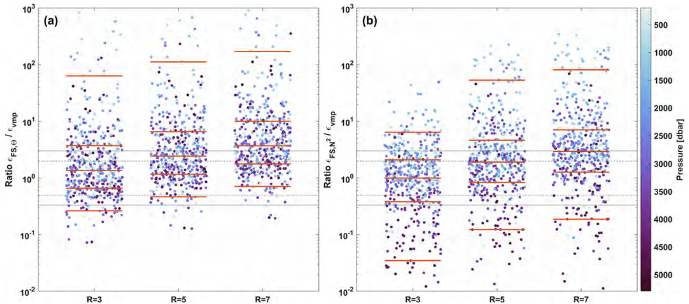
Figure 4. The ratios between \varepsilon_{FS} and \varepsilon_{vmp} , for different values of R_\omega . With (a) strain based on \Theta_z and (b) strain based on N^2 . \varepsilon_{vmp} has been averaged over the same segments as the segments of the finescale method. Color coding of the dots indicates average pressure of finescale estimate. The black lines indicate a factor 2 (dashed) and 3 (dotted) respectively, and the orange lines mark, from bottom to top, the 5, 25, 50, 75 and 95th percentiles. Jitter of the dots is to increase readability.
