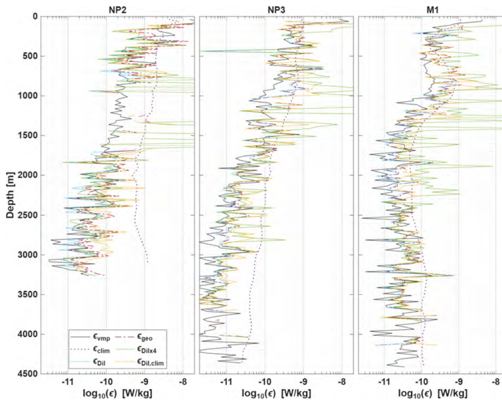
Figure C3. Dissipation estimates \varepsilon_{\text{TP}} for all different methods ( \varepsilon_{\text{geo}} : Method 1, \varepsilon_{\text{Dil}} : Method 2, \varepsilon_{\text{Dilx4}} : Method 3 and \varepsilon_{\text{Dil,clim}} : Method 4, as defined in Sect. 5.4) are compared to \varepsilon_{\text{vmp}} and the used climatological estimates \varepsilon_{\text{clim}} , shown for three example stations.
